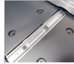
HELICAL-STYLE CUTTER HEAD W/ 12 TWO-SIDED CARBIDE INSERTS
